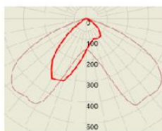
Type II (50°x140°)
